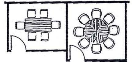
10' X 12' / 120 SF
